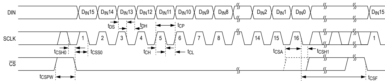
Figure 2. SPI Timing Diagram
