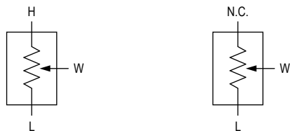
Figure 1. Voltage-Divider and Variable Resistor Configurations
