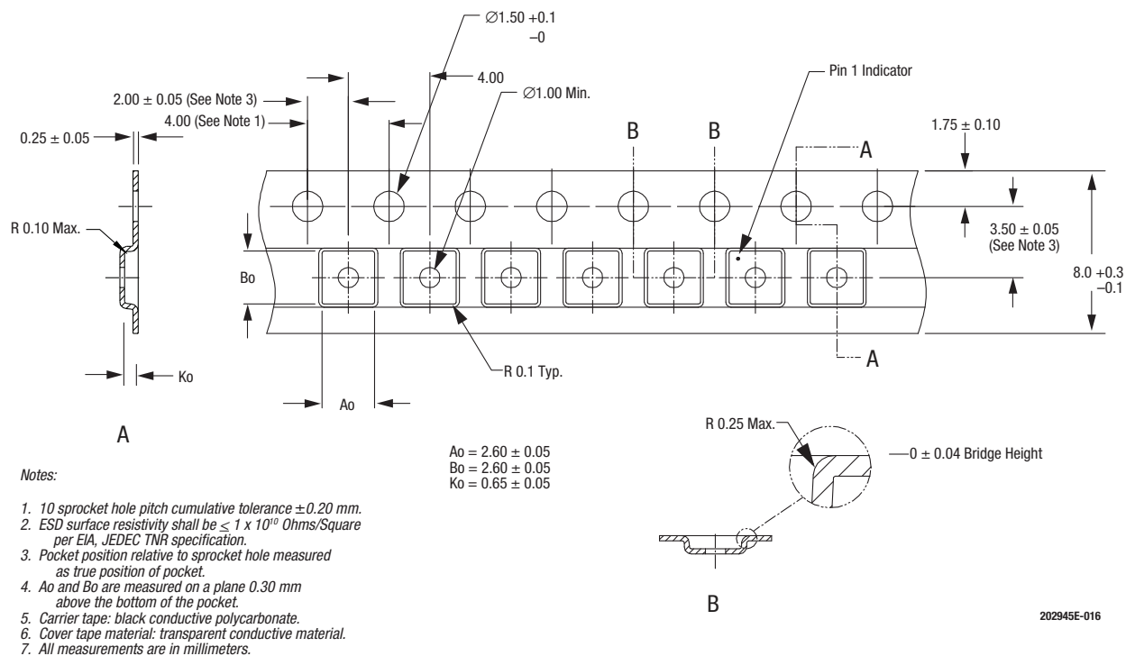
Figure 16. SKY16602-632LF Tape and Reel Dimensions
