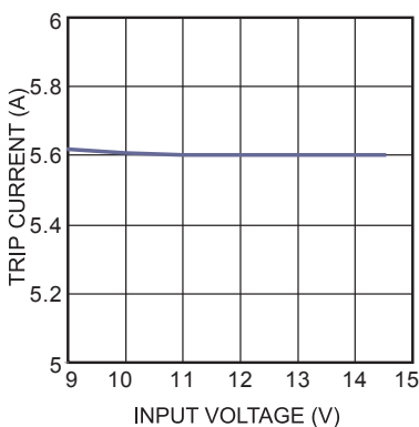
Trip Current vs. Input Voltage
