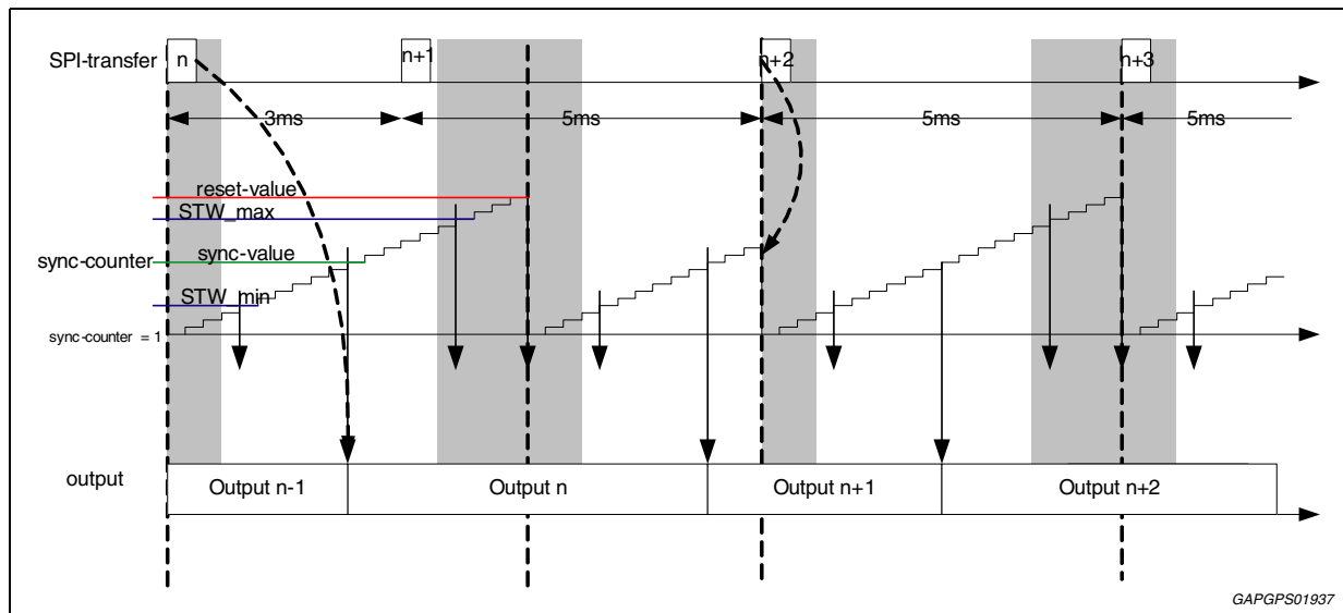
Figure 16. Sync-failure + re-synchronization
