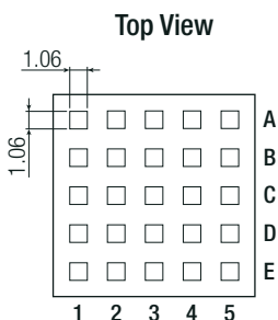
Recommended Footprint Details
