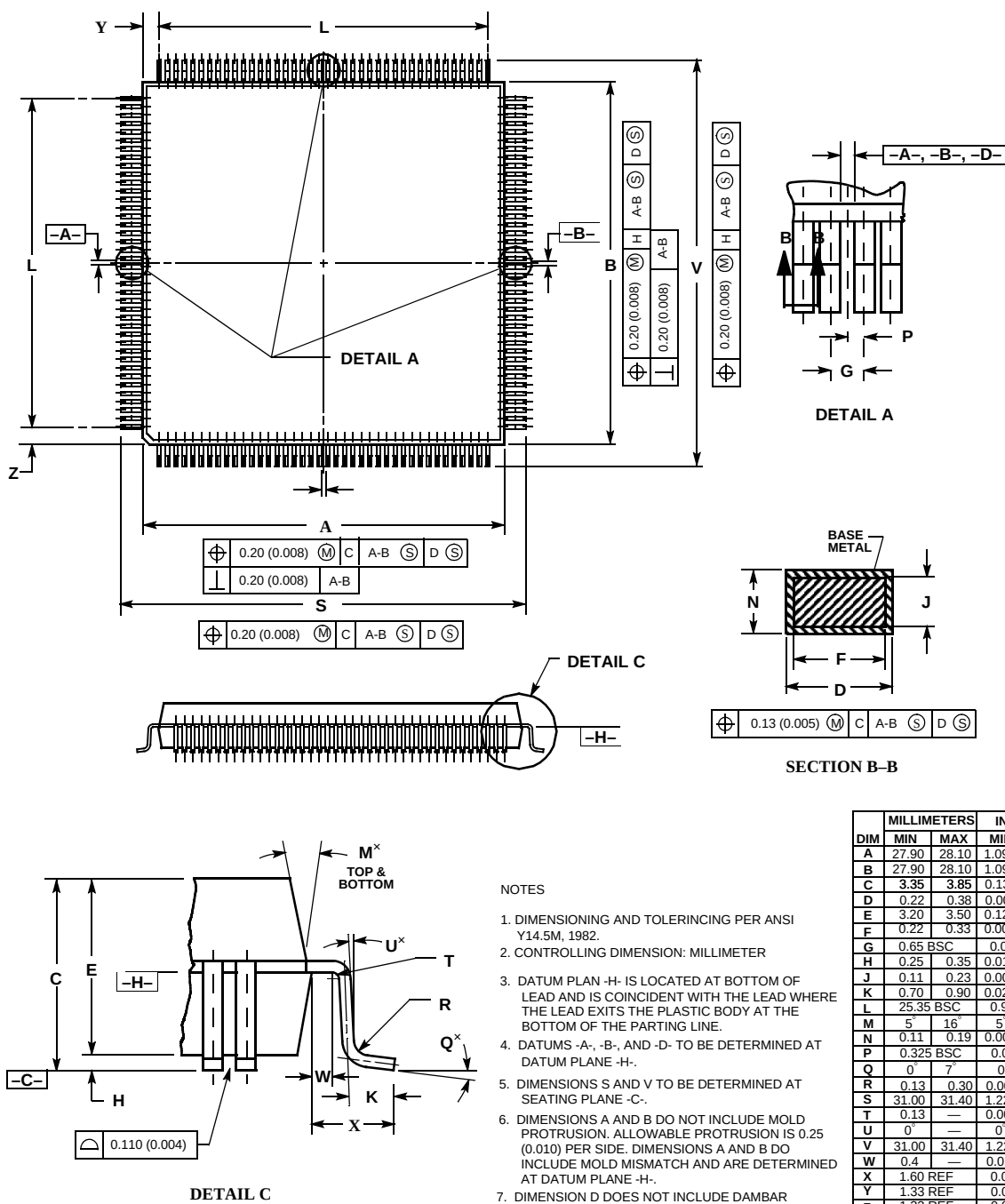
Case 864A-03 Figure 6. 160 QFP Package Dimensions
