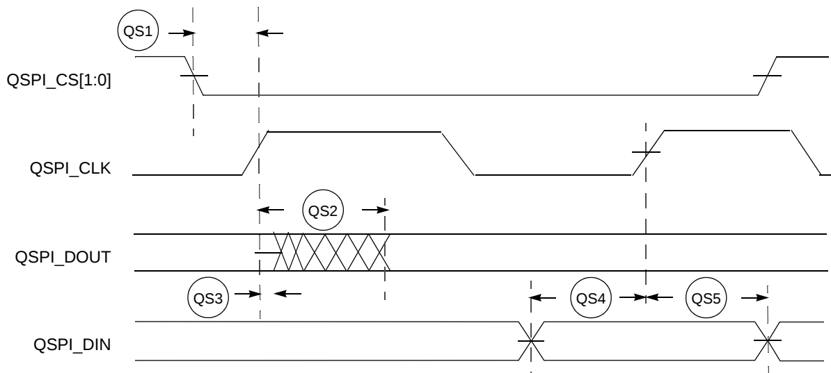
Figure 20. QSPI Timing
