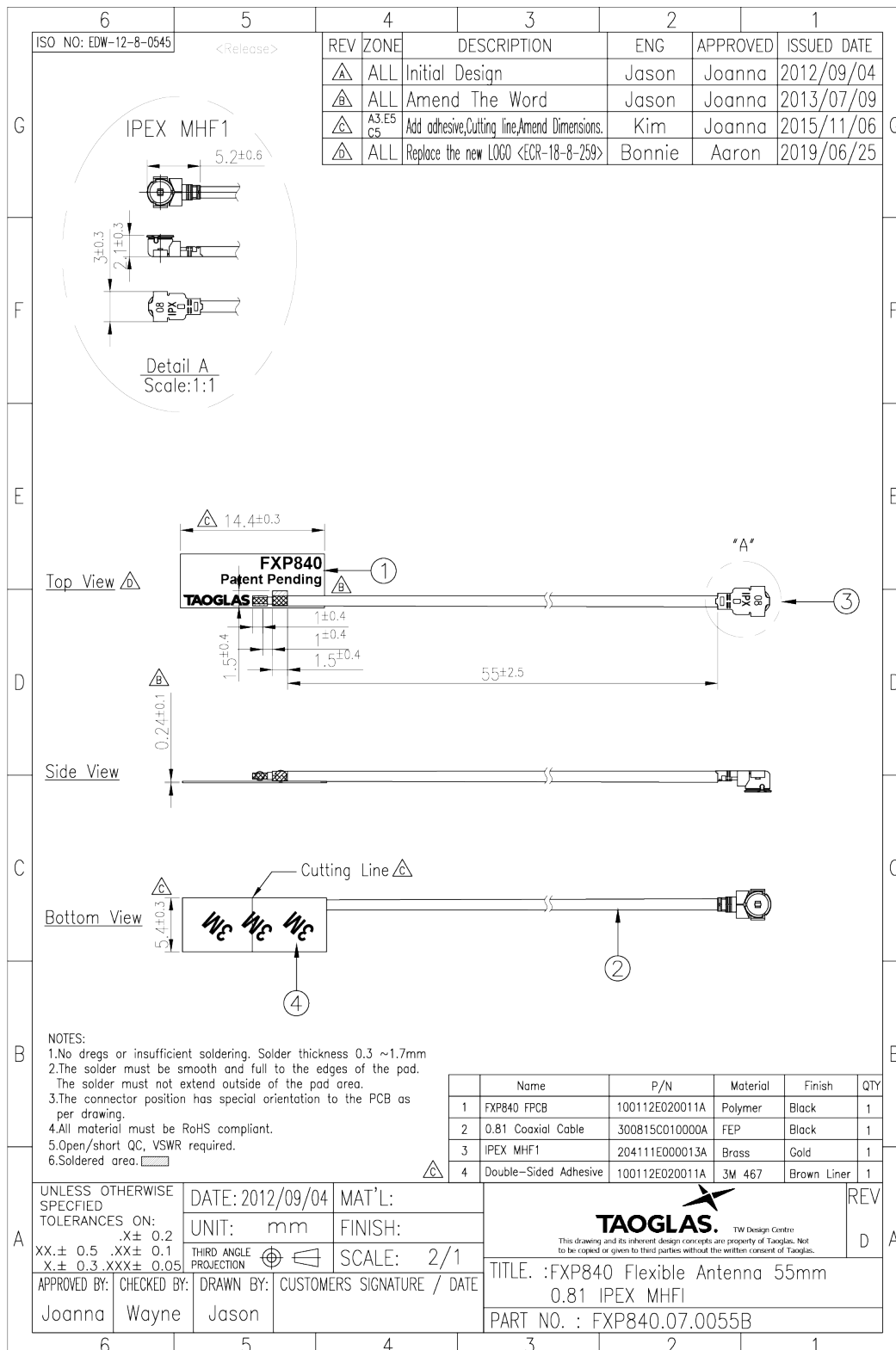
Figure 15. Antenna Drawing.
