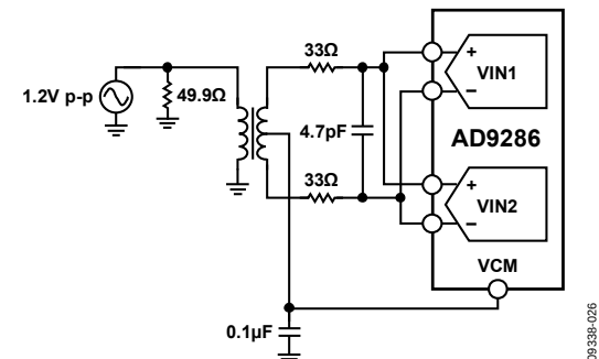
Figure 25. Differential Transformer-Coupled Configuration
