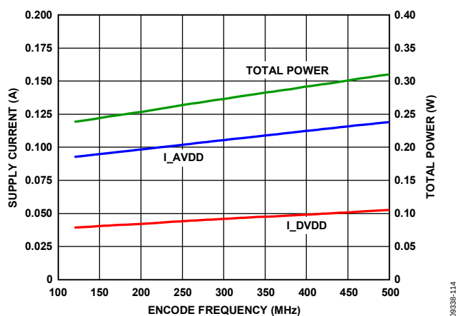
Figure 14. Supply Current and Power vs. Encode
