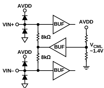
Figure 19. Analog Inputs ( V_{CML} \approx 1.4\text{ V} )
