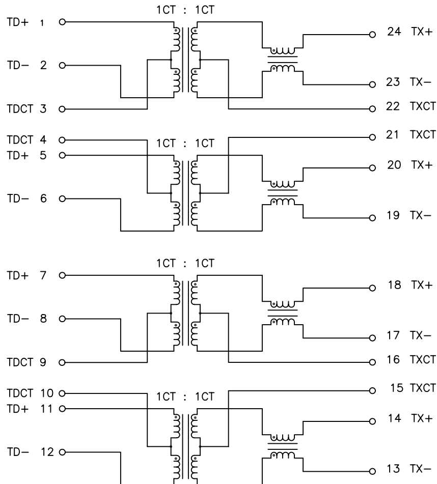
SCHEMATIC
