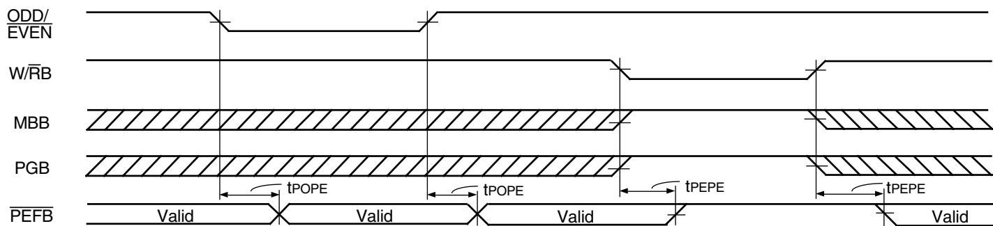
Figure 18. ODD/ \overline{\text{EVEN}} W/ \overline{\text{RB}} , MBB, and PGB to \overline{\text{PEFB}} Timing
