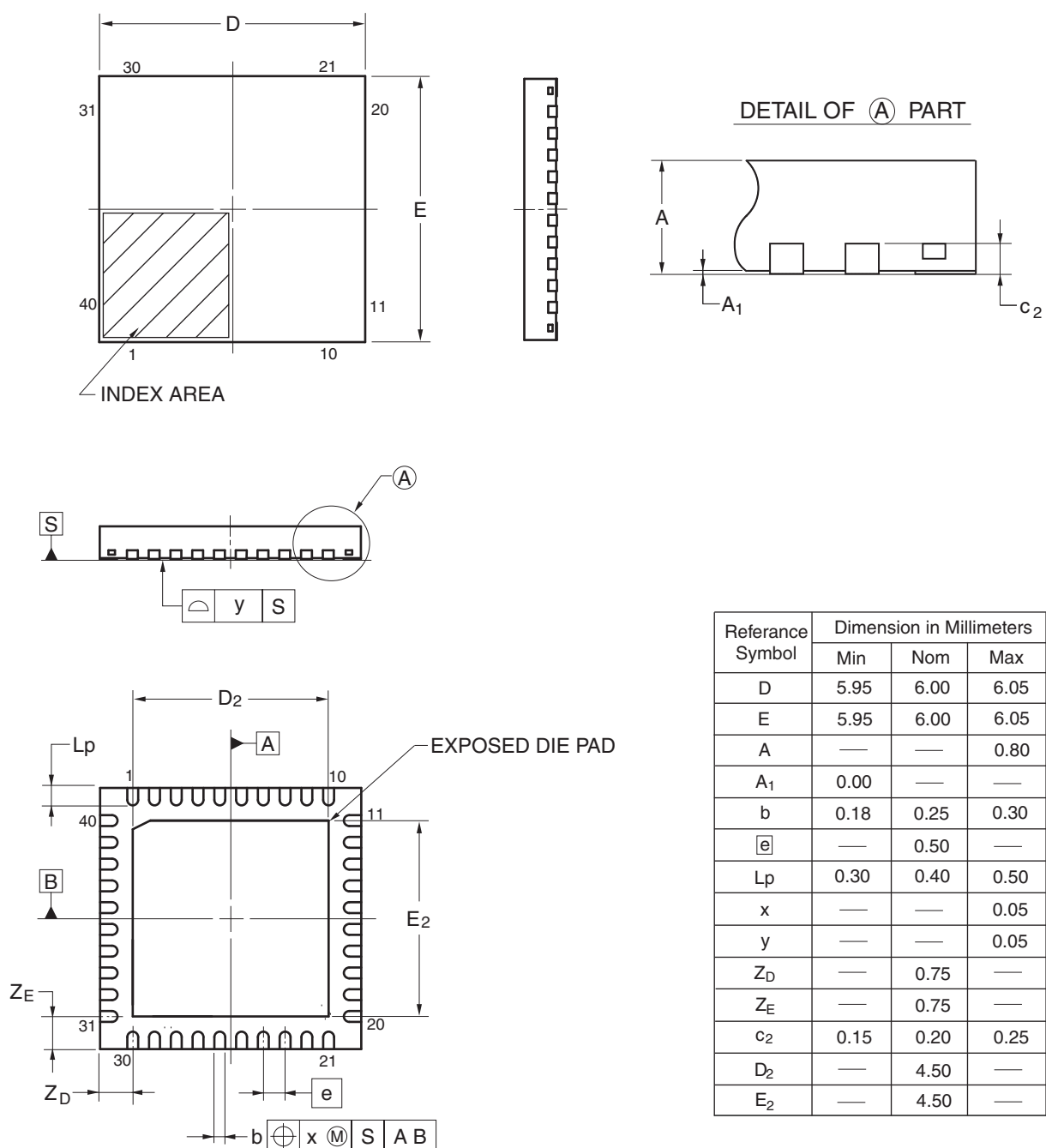
Figure 1.5 QFN 40-pin
