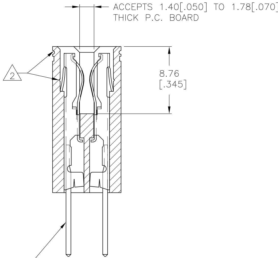
CONTACTS SHOWN FOR REF ONLY SECTION Z-Z
