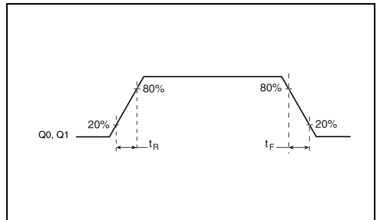
Single-Ended Output Rise/Fall Time
