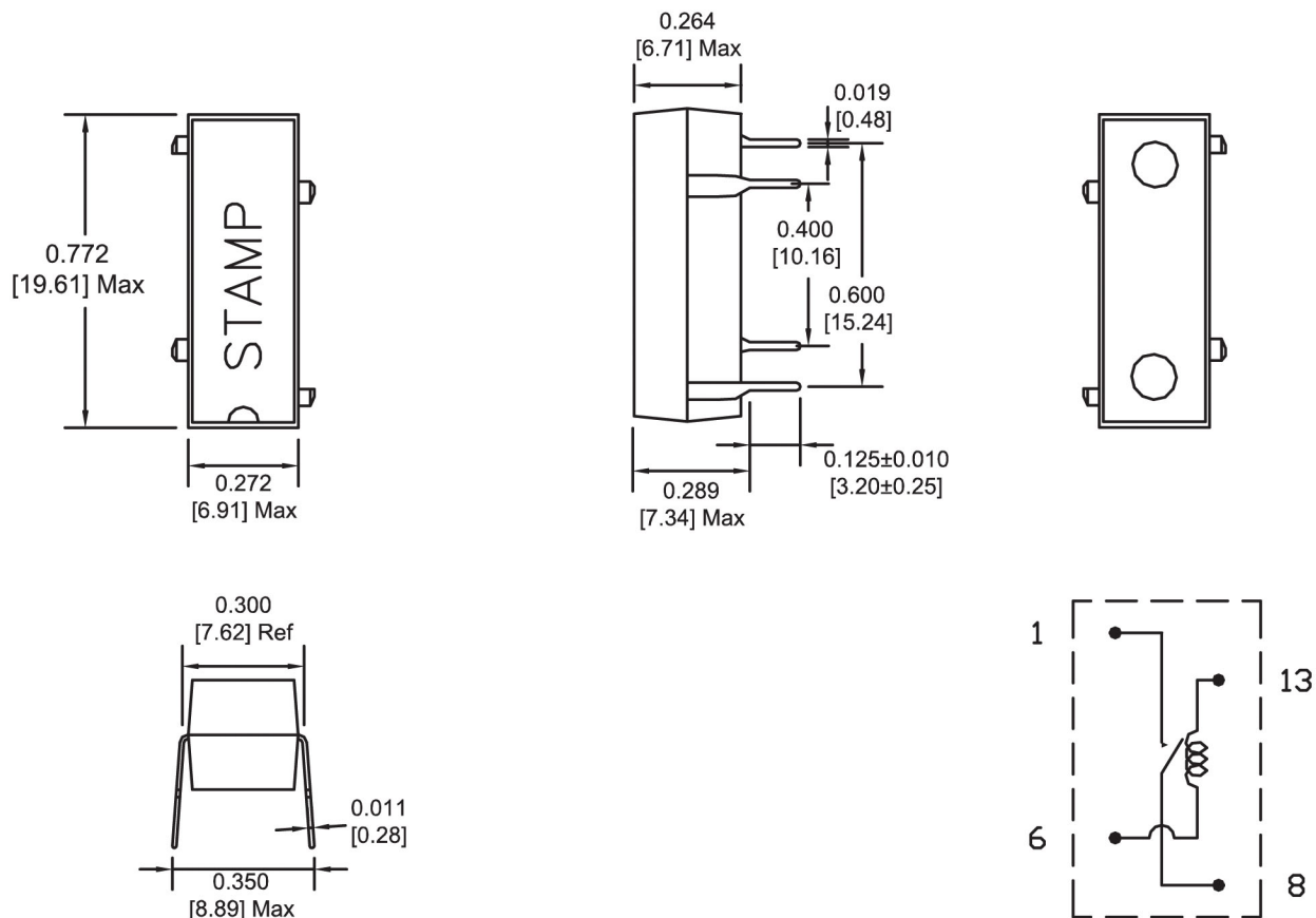
WIRING DIAGRAM
