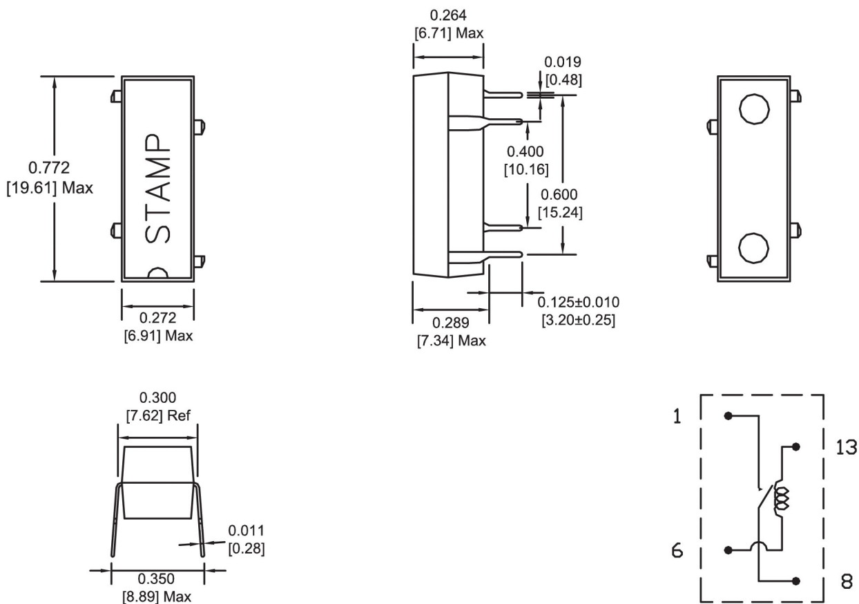
WIRING DIAGRAM
