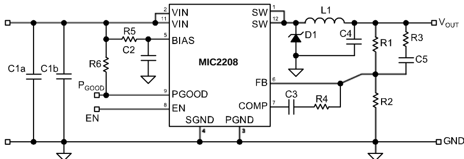
MIC2208 Evaluation Board Schematic
