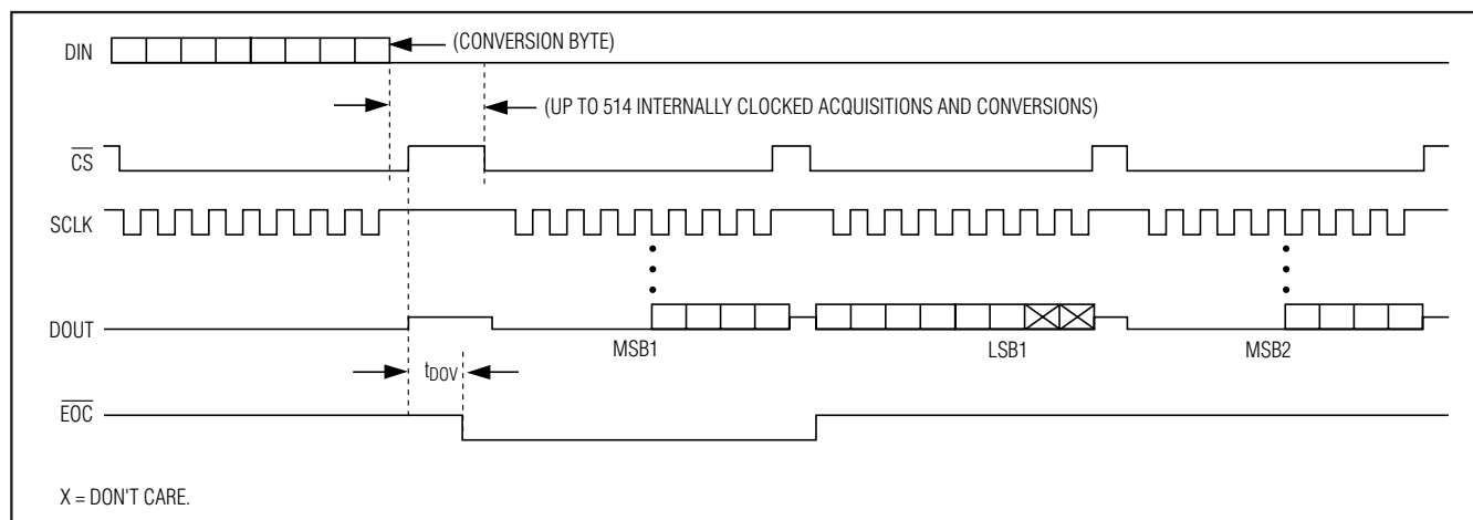
Figure 8. Clock Mode 10—The command byte to the conversion register begins the acquisition ( \overline{\text{CNVST}} is not required).
