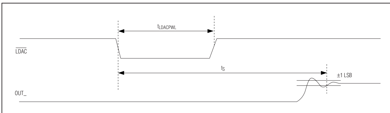
Figure 14. LDAC Functionality
