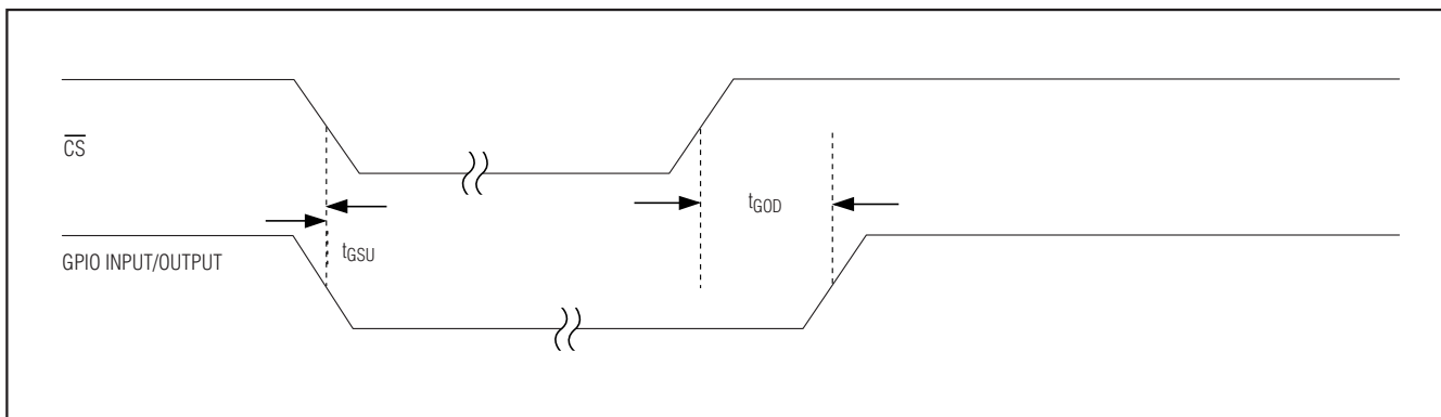
Figure 13. GPIO Timing
