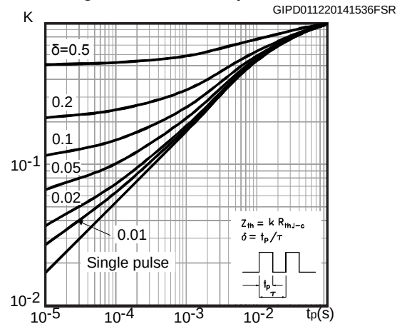
Figure 3: Thermal impedance
