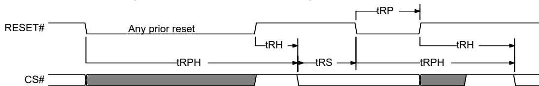
Figure 139. Hardware Reset using RESE# Input
