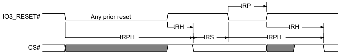
Figure 140. Hardware Reset when Quad or QPI Mode is not enabled and IO3 / RESE# is Enabled
