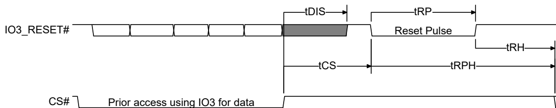
Figure 141. Hardware Reset when Quad or QPI Mode and IO3 / RESE# are Enabled
