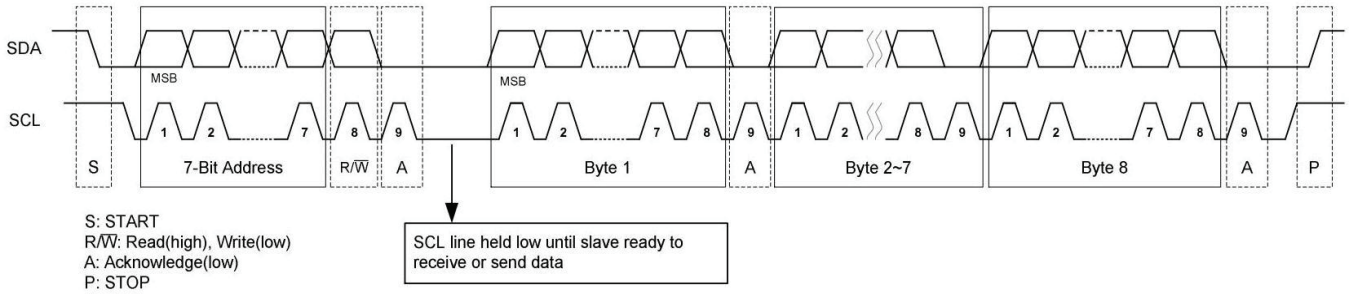
I2C Waveform
