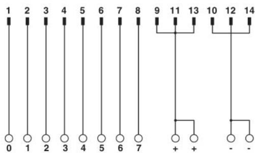
Circuit diagram
