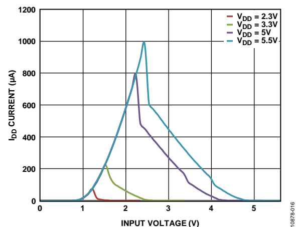
Figure 16. I_{DD} Current vs. Digital Input Voltage
